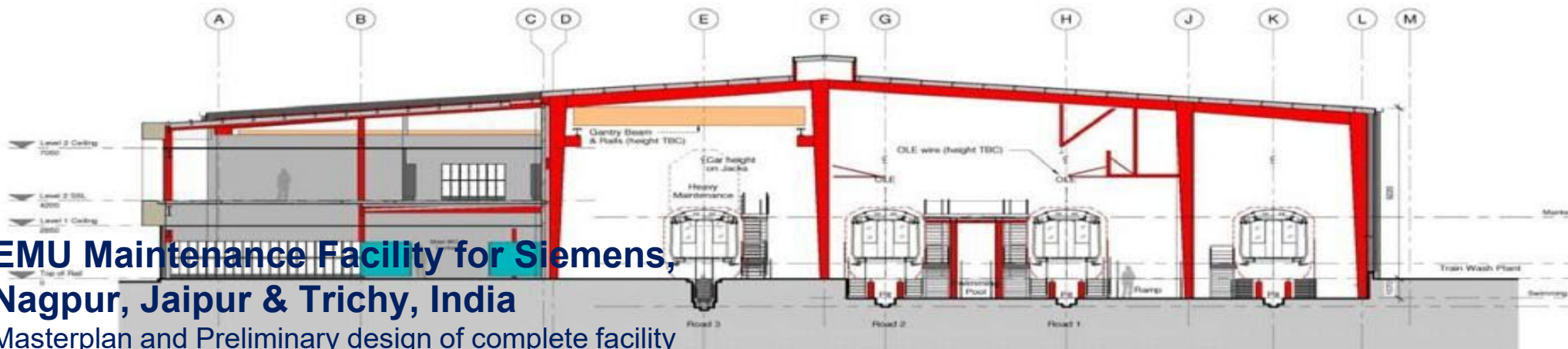
Main Depot Section A-A
