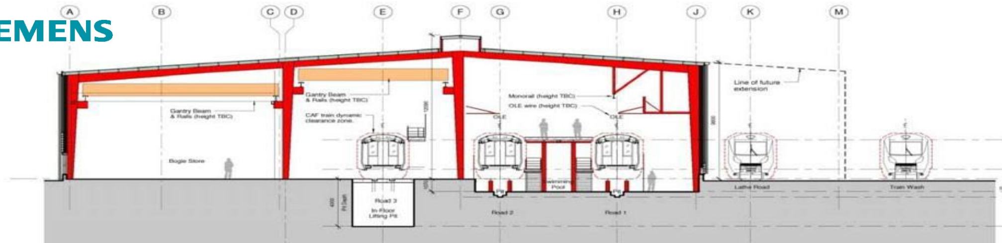
2 Main Depot Section B-B 1 : 100
